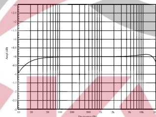
Figure 9. Frequency response
