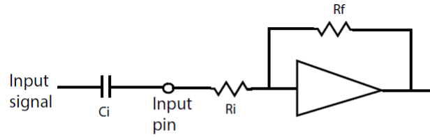
Figure 22. Input circuit and frequency response
